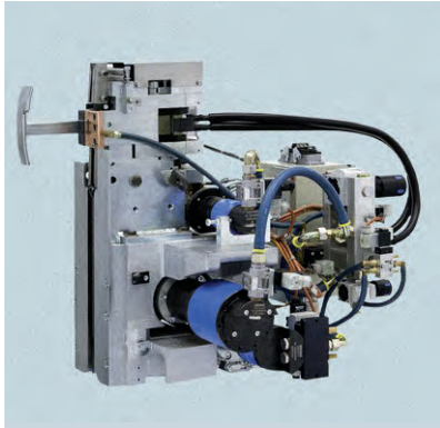
Hydraulically actuated down ender
